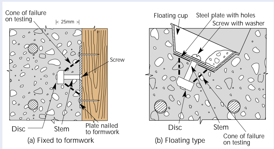
Figure 3: Lok-test inserts.
